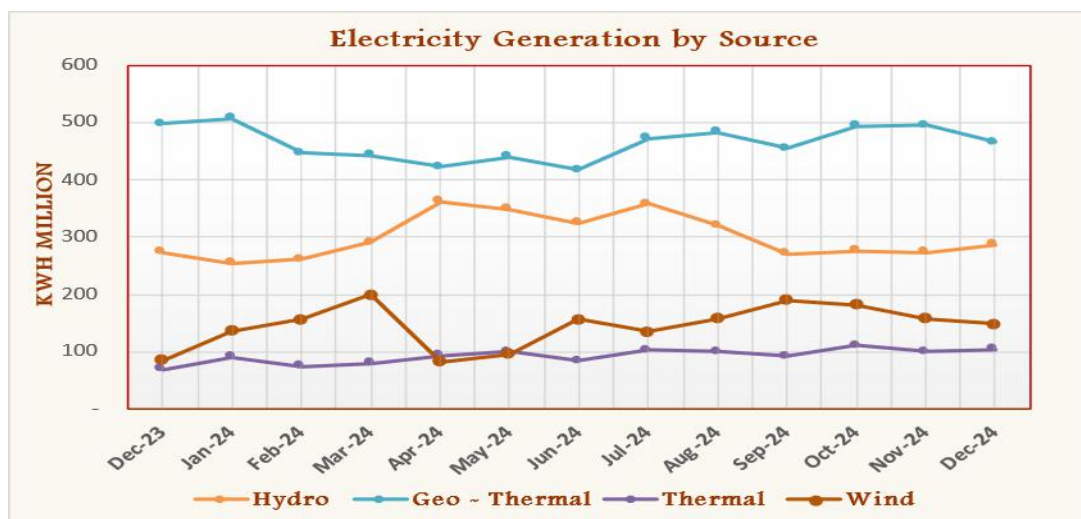
Figure 7: Electricity Generation by Source
