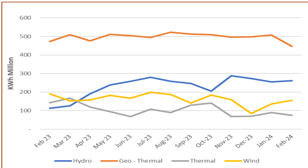
Figure 7: Electricity Generation by Source
